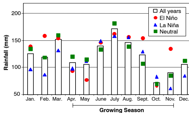
Figure 1. Historical (1950–2004) monthly rainfall in Jackson County, Florida, for El Niño, La Niña, and neutral ENSO phases compared to all years (source: www.agclimate.org).
