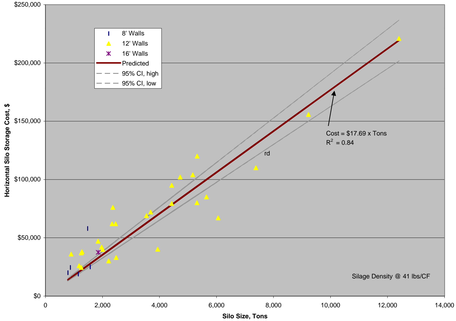
Horizontal Silo Storage Cost vs Tons Stored
