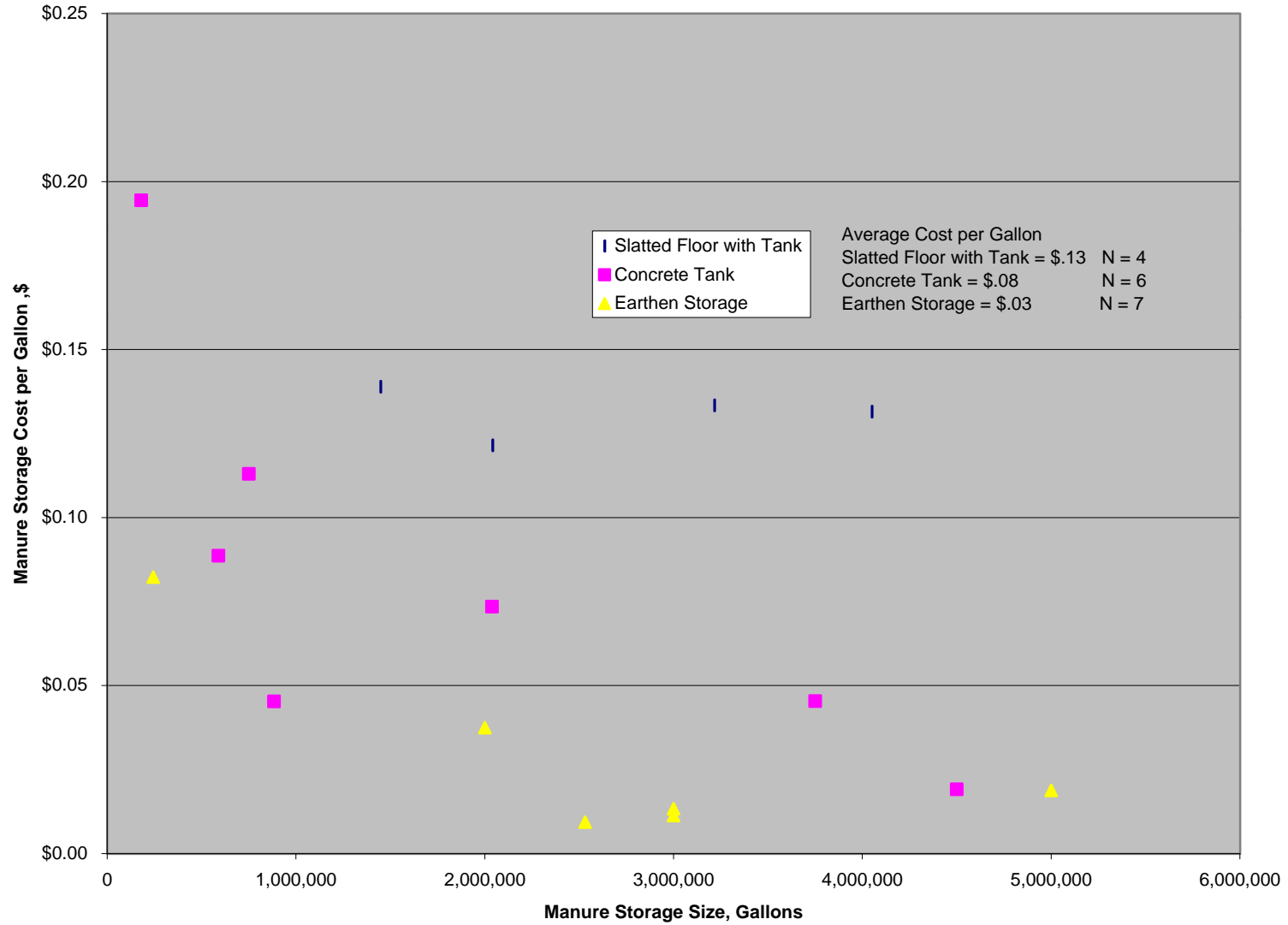
Manure Storage Cost per Gallon vs Size
