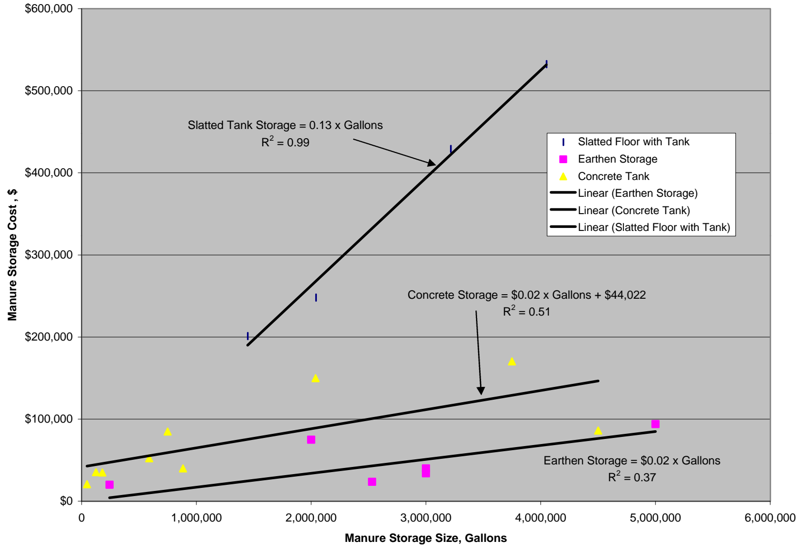
Manure Storage Cost vs Size
