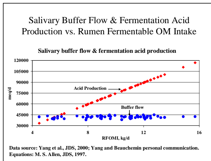
Figure 2. Calculated fermentation acid production and salivary buffer flow at varying intakes of rumen-fermentable organic matter.
