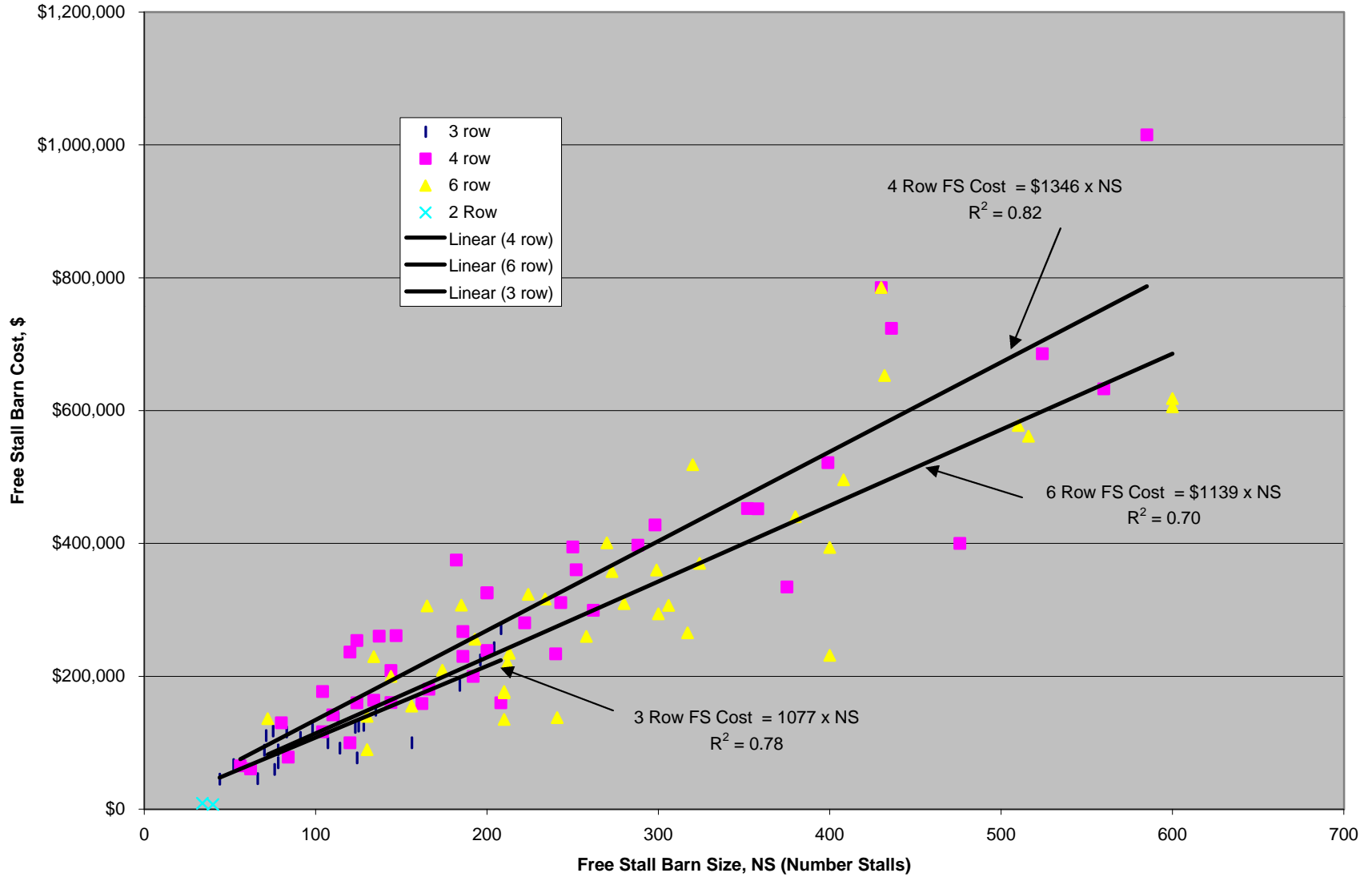
Free Stall Barn Cost vs Free Stall Barn Size
